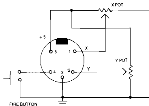
Figure 1: Radio Shack Joystick
