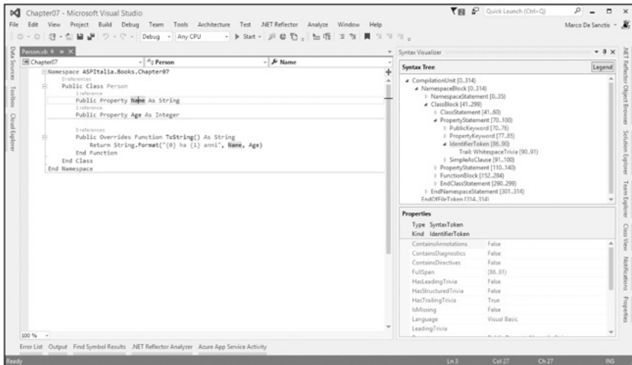
Figura 7.6 – Syntax Visualizer in Visual Studio 2015.
