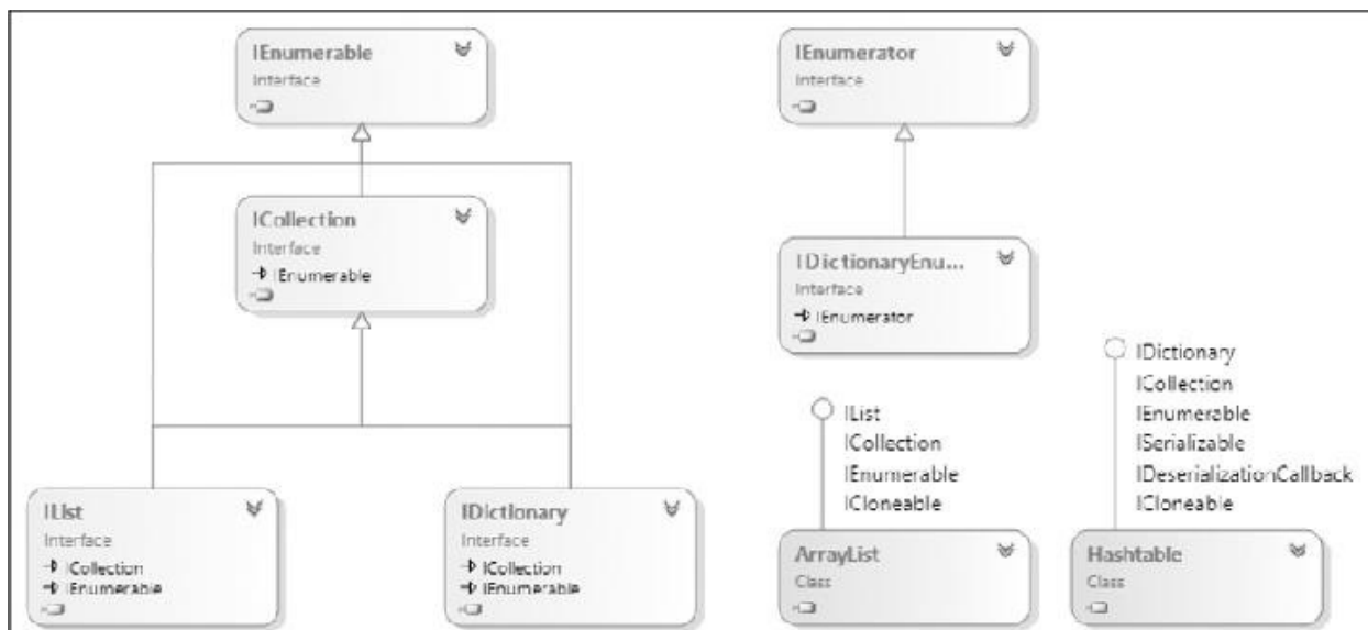
Figura 5.1 – Interfacce e classi in System.Collections.
