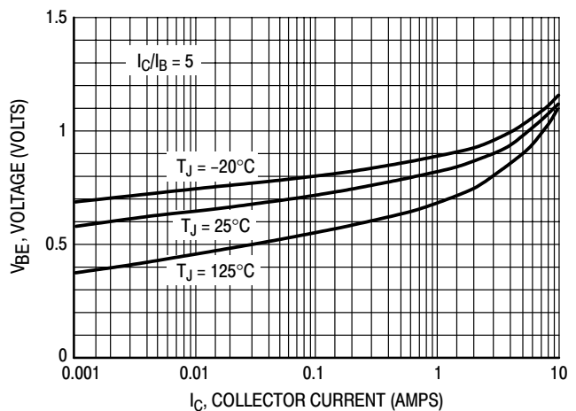
Figure 24. Base-Emitter Saturation Region
