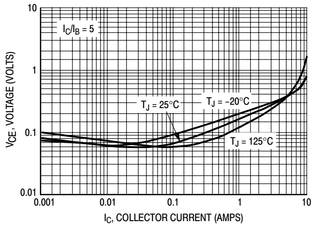
Figure 22. Collector-Emitter Saturation Voltage
