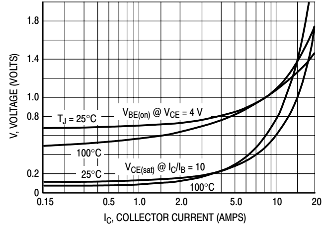
Figure 5. "On" Voltage
