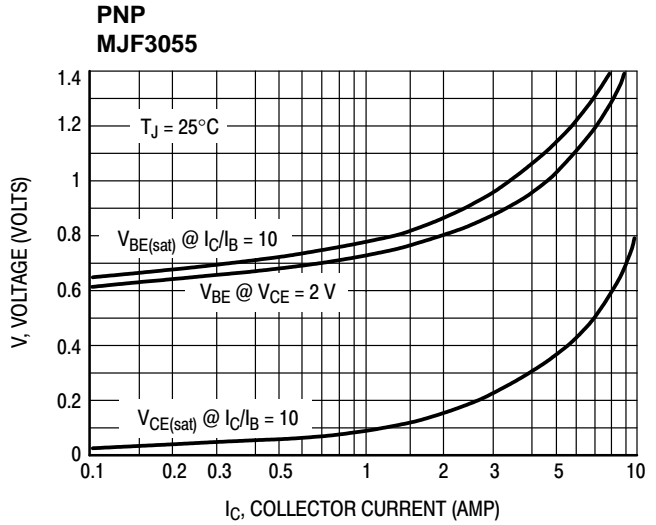
Figure 9. "On" Voltages
