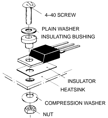
Figure 25. Screw-Mounted TO-220
