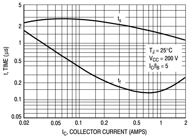
Figure 8. Turn-Off Time
