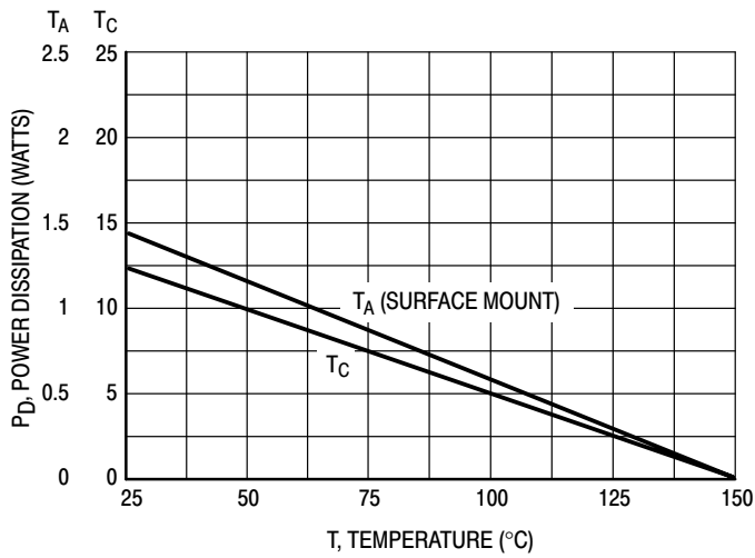
Figure 34. Power Derating
