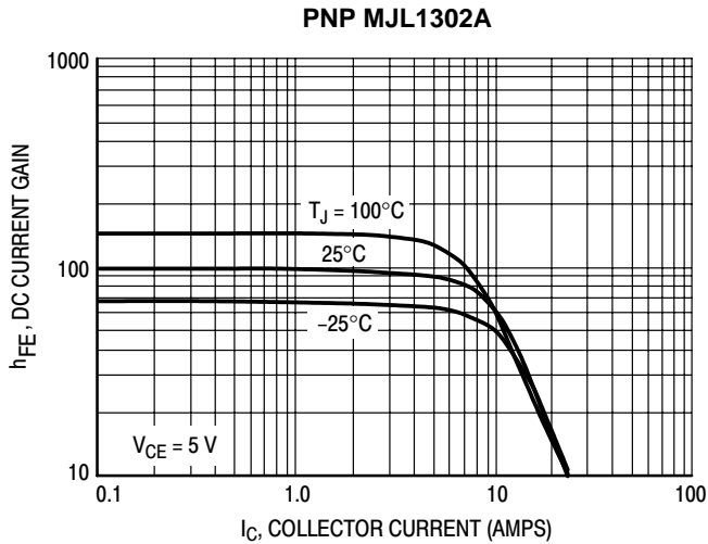
Figure 22. DC Current Gain, V_{CE} = 5\text{ V}
