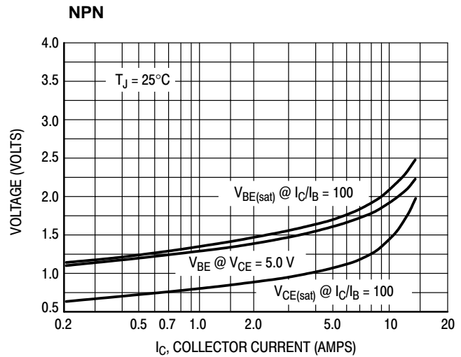
Figure 8. "On" Voltages
