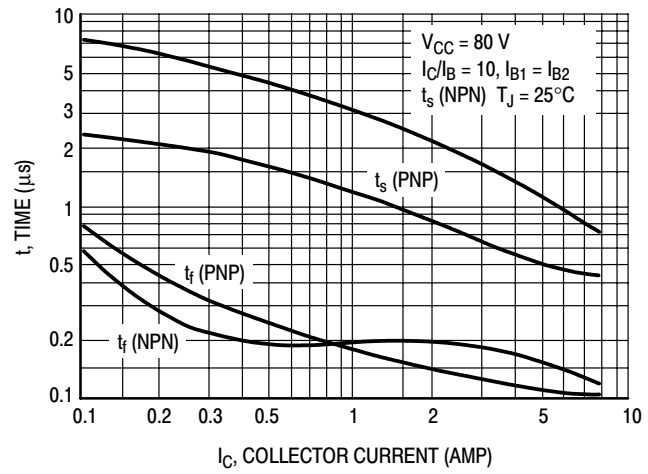
Figure 10. Turn-Off Times
