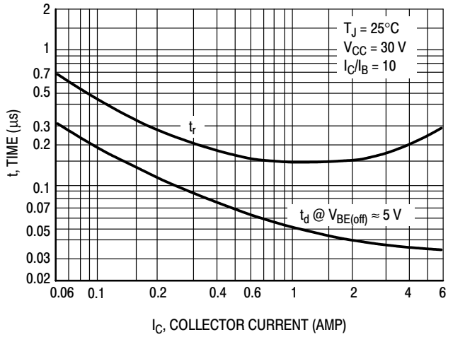
Figure 11. Turn-On Time
