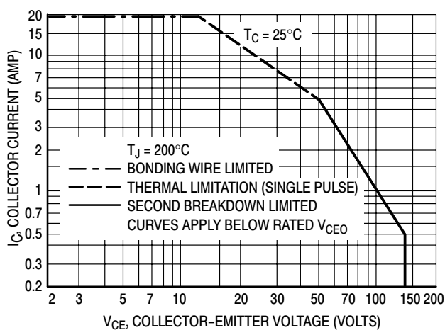
Figure 1. Active-Region Safe Operating Area
