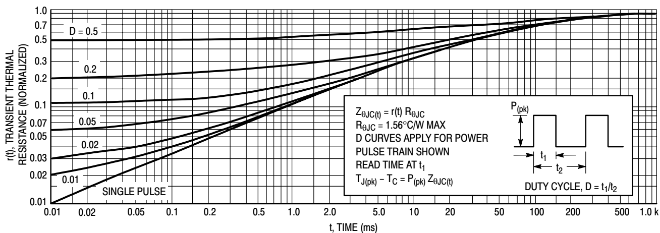
Figure 2. Thermal Response
