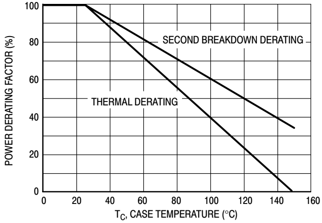
Figure 11. Power Derating
