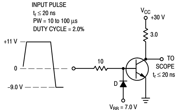
Figure 3. Turn–Off time
