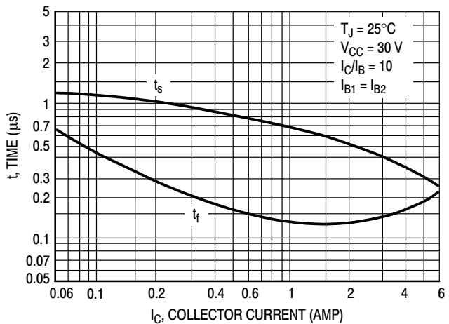
Figure 13. Turn-Off Time
