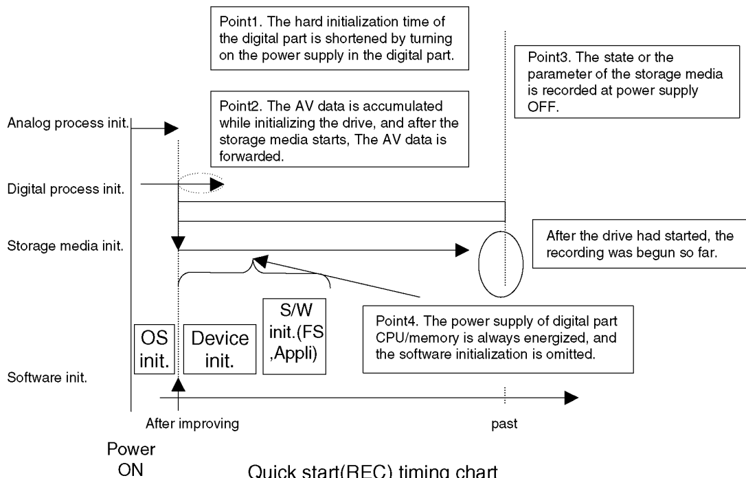
Quick start(REC) timing chart
