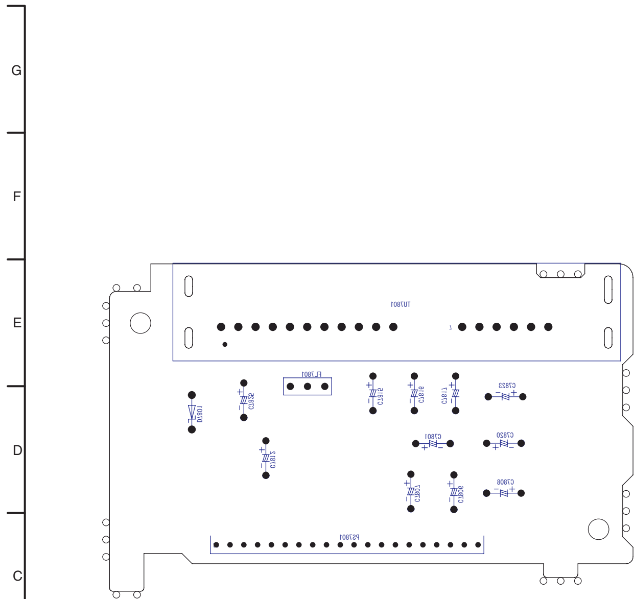
(Component Side)
