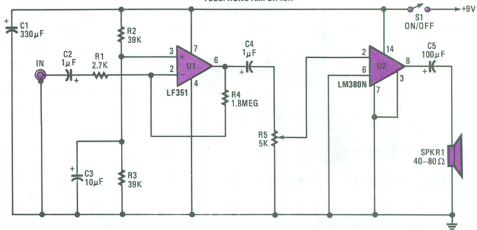
TELEPHONE AMPLIFIER
