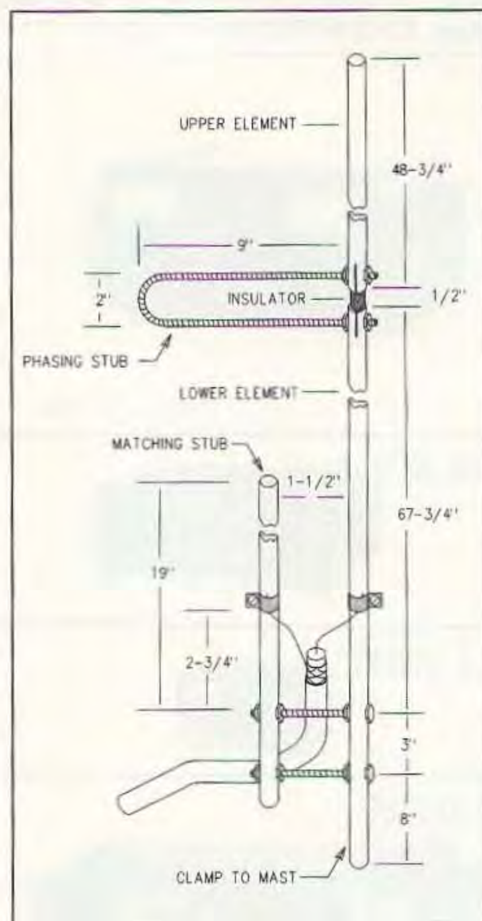
Figure 2. Construction details.
