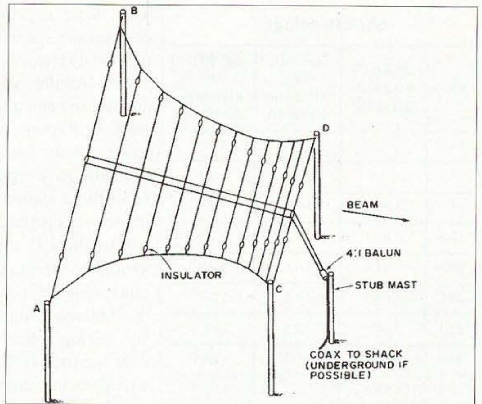
Fig. 4. For method of transposing the center feeder see Fig. 1(b) and Fig. 6. Illustrates the four masts used to support the antennas.
