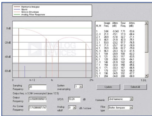
Figure 11. Screen presentation provided by an interactive design tool. A \sin(x)/x presentation of a typical device output.
