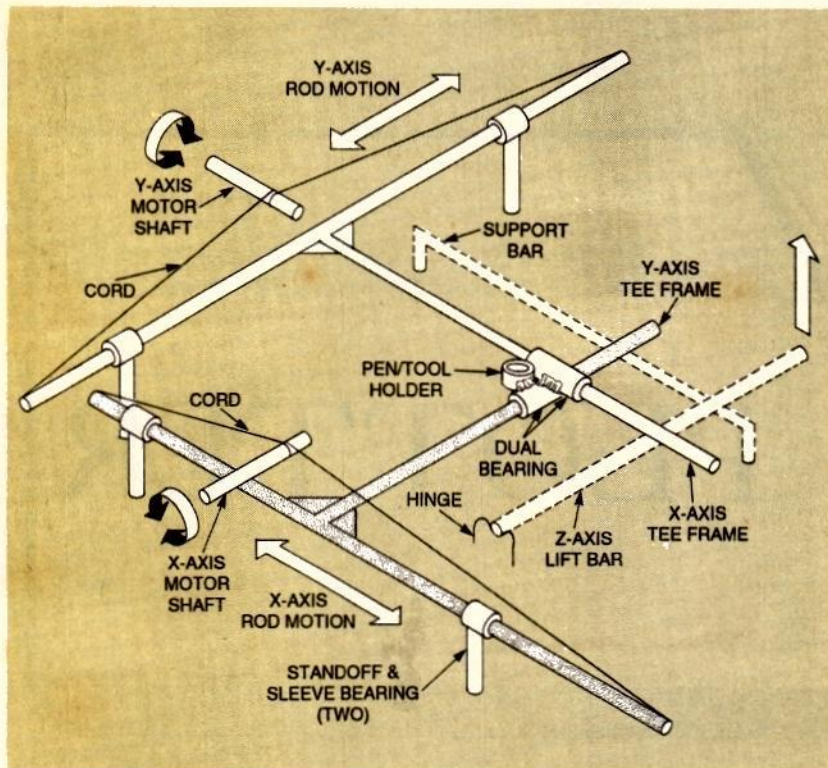
FIG. 1—CONCEPT OF X-Y PLOTTER. A pen in the holder coupled to two overlapping X and Y tee frames is driven in two degrees of freedom. The holder resolves the simultaneous winching actions of the X and Y stepper motors.
