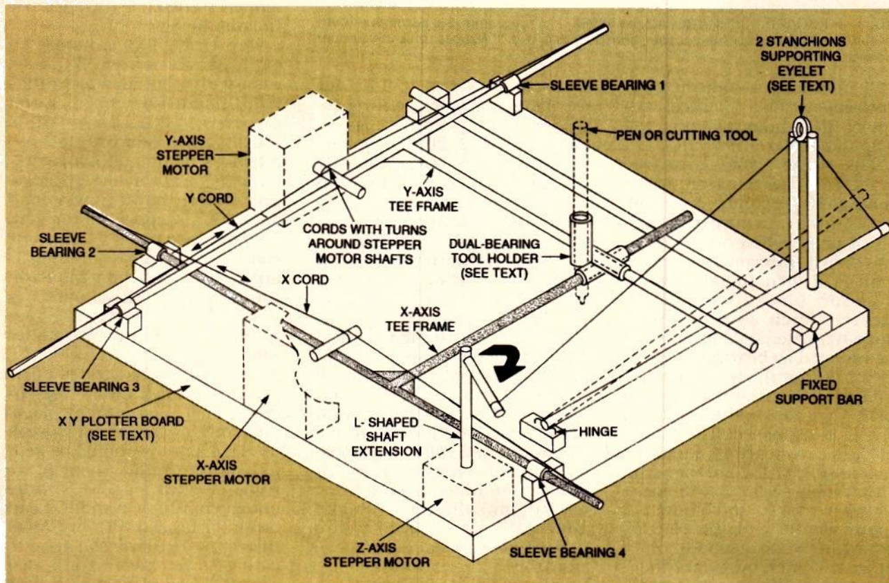
FIG. 2—CONSTRUCTION DETAILS OF X-Y PLOTTER. The tee frames can be made from different kinds of light, strong materials, but they must be slide easily in their sleeve-bearing supports without binding. The vertically mounted Z-axis motor lifts the X and Y arms and tool holder when a crank arm pulls on the cord attached to the side rail.
