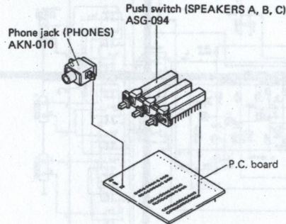
Switch Assembly (AWS-095)
