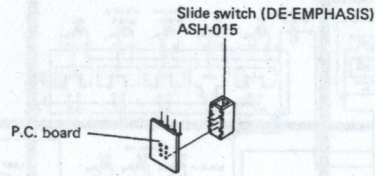
Switch Assembly (AWX-095)
