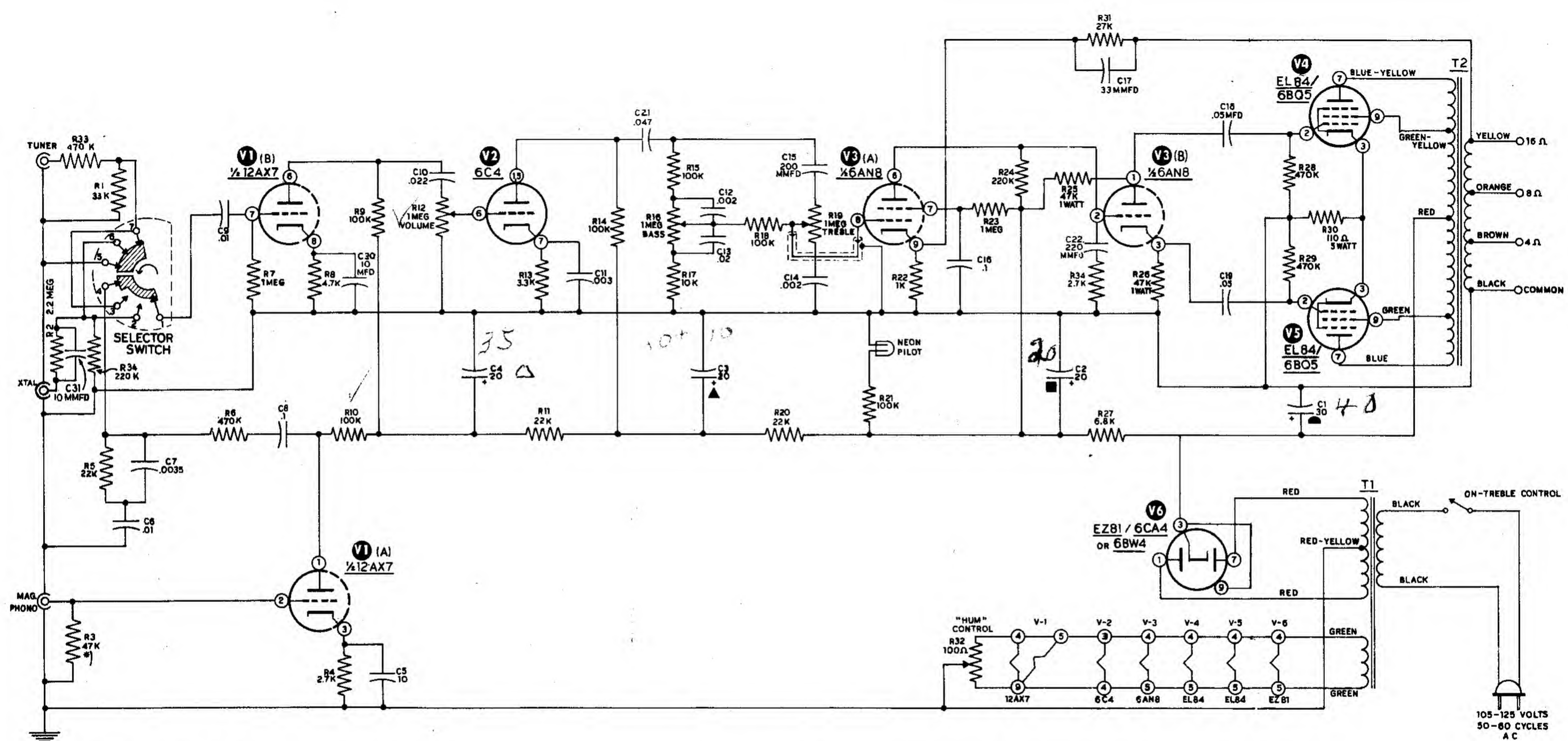
SCHMATIC HEATHKIT HIGH FIDELITY 12 WATT AMPLIFIER MODEL EA-2
