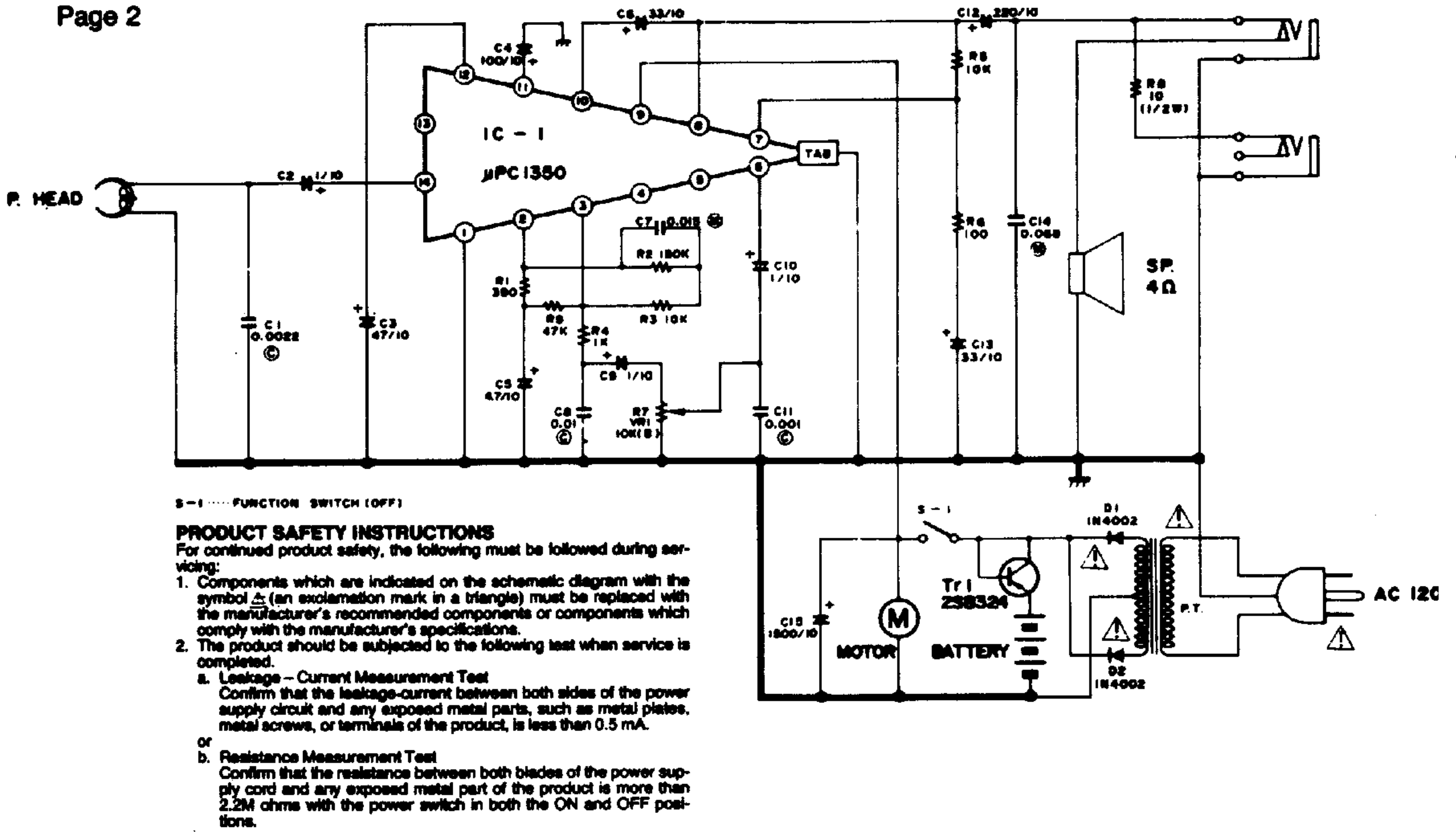
SCHEMATIC, MODEL 3110
