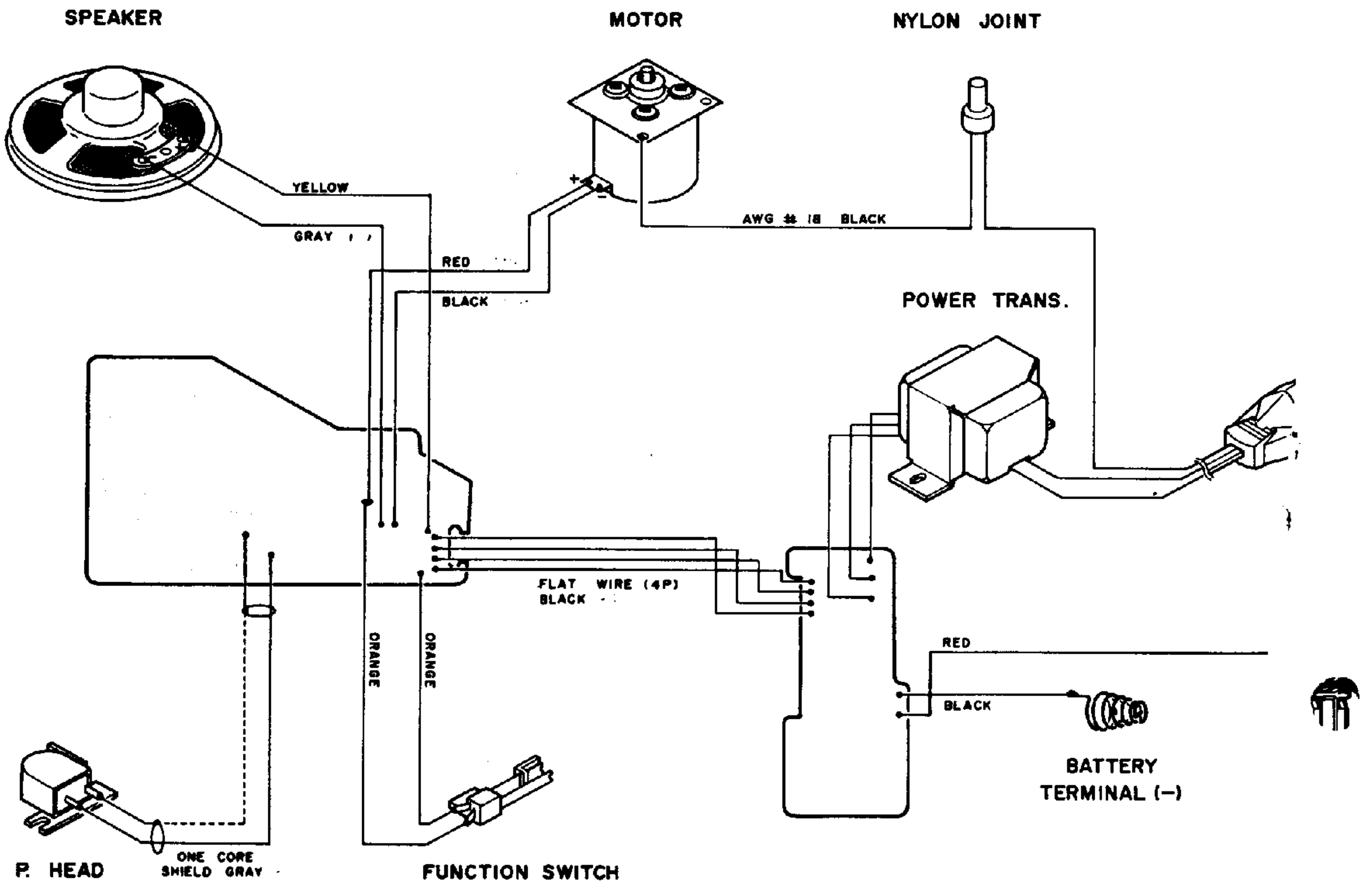
WIRING, MODEL 3110
