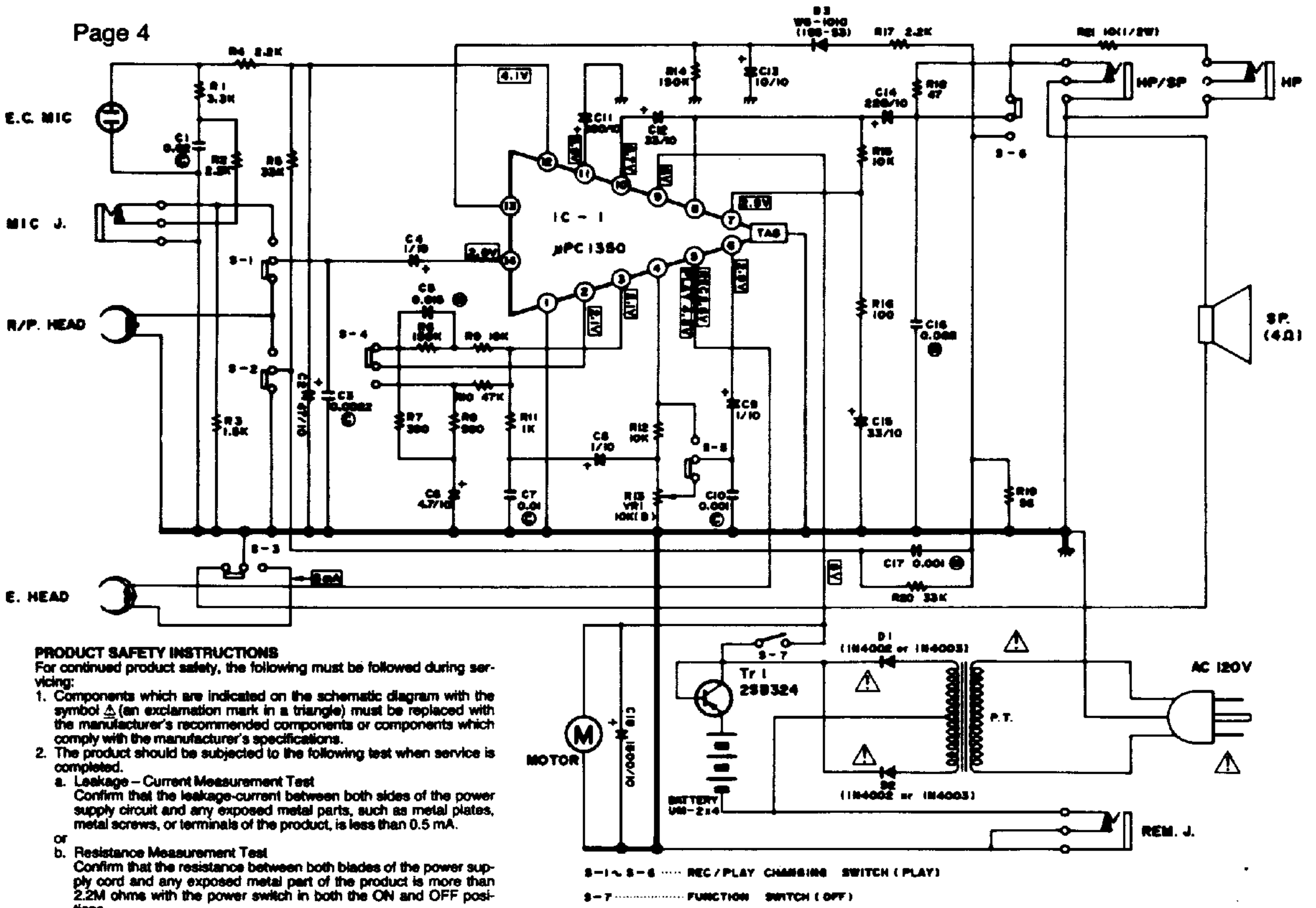
SCHEMATIC, MODEL 3130
