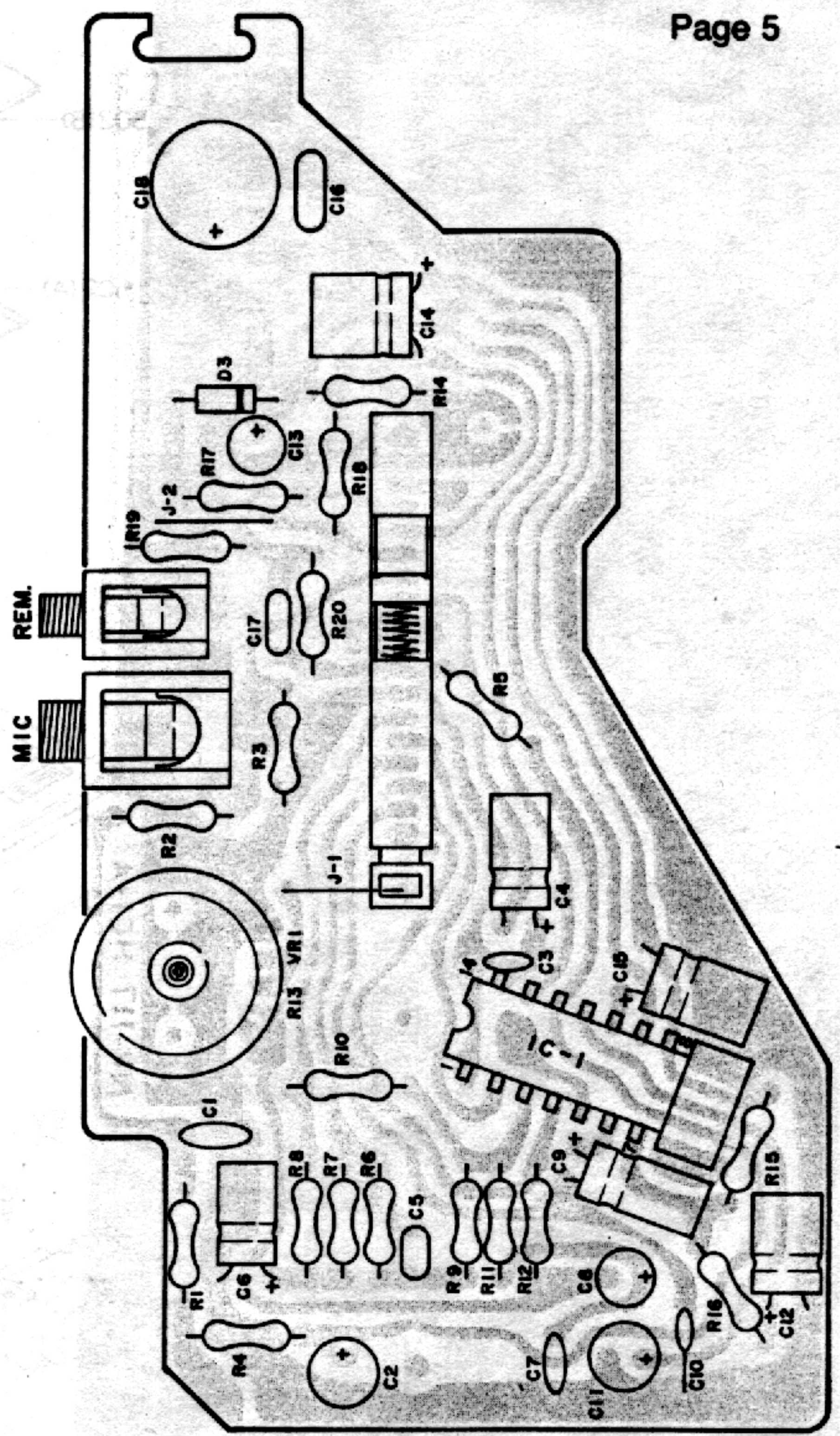
MODEL 3130 MAIN PC BOARD
