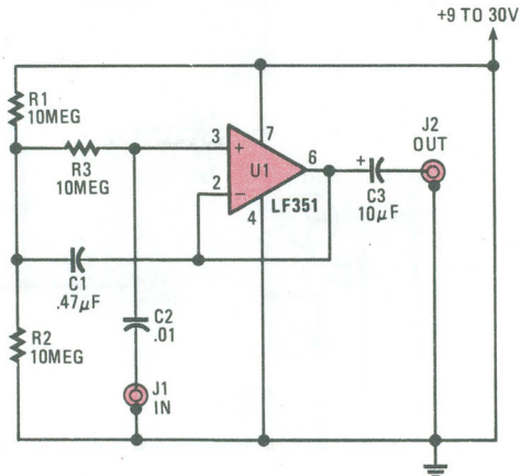
HIGH IMPEDANCE BUFFER AMPLIFIER
