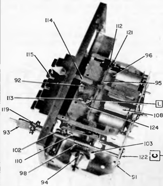
TUNER
