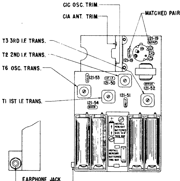
TRANSISTOR & TRIMMER LAYOUT FOR 7AT42Z1
