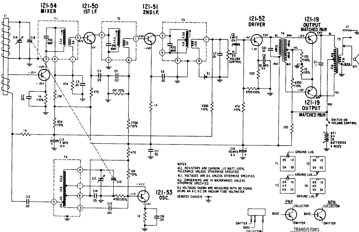
SCHEMATIC DIAGRAM FOR 7AT42Z1
