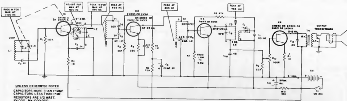
P710A, P711A
