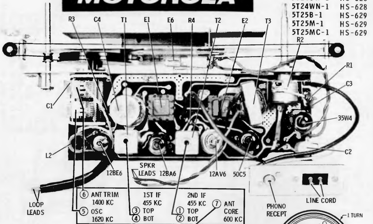
ANTENNA CIRCUIT INDUCTANCE ADJUSTMENT
