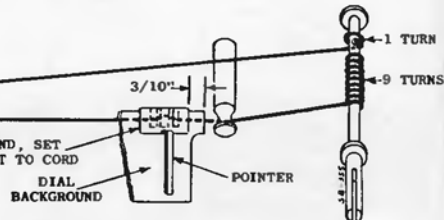
DIAL RESTRINGING DETAIL
