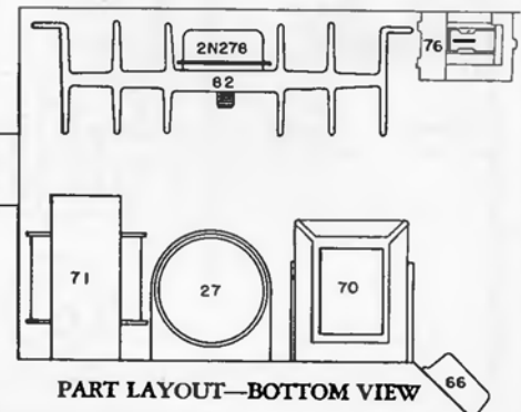
NUMBERS ON PRINTED CIRCUIT BOARD CORRESPOND WITH NUMBERS IN CIRCLES ON SCHEMATIC DIAGRAM.
