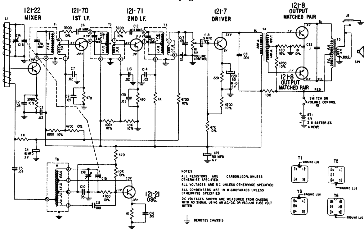
SCHEMATIC DIAGRAM FOR 7AT42
