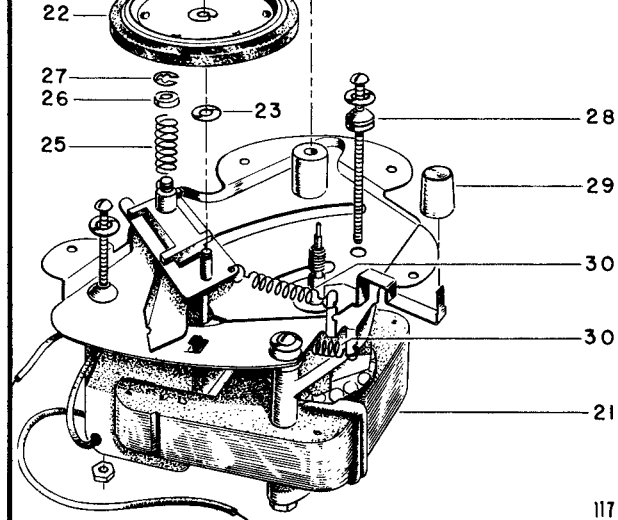
Exploded View of Motor and Turntable.
