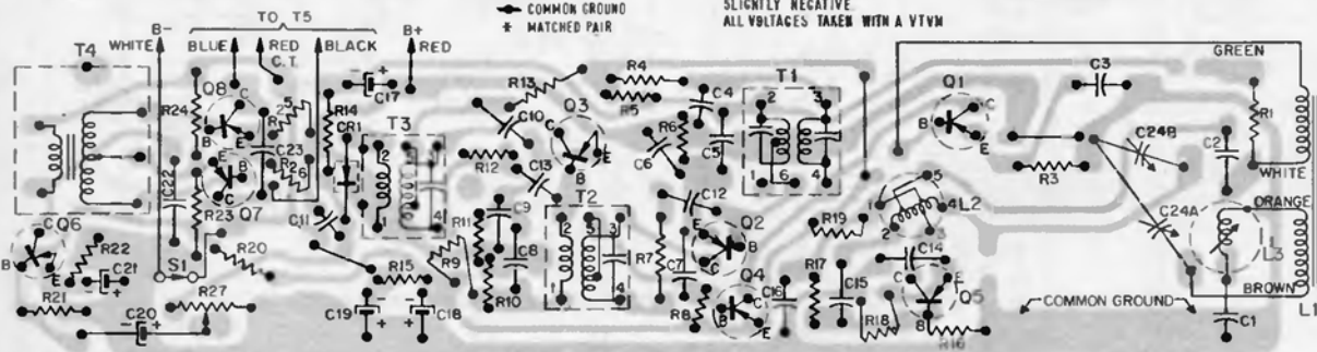
View of Printed Wiring Board. NOTE: Gray area represents printed wiring, black symbols and lines represent components and wiring on opposite side.
