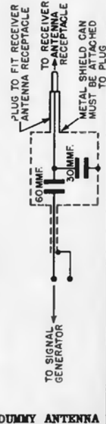
DUMMY ANTENNA
