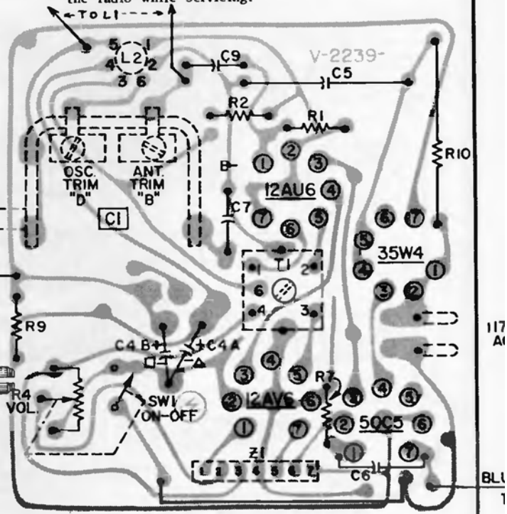
BOTTOM VIEW OF CHASSIS
