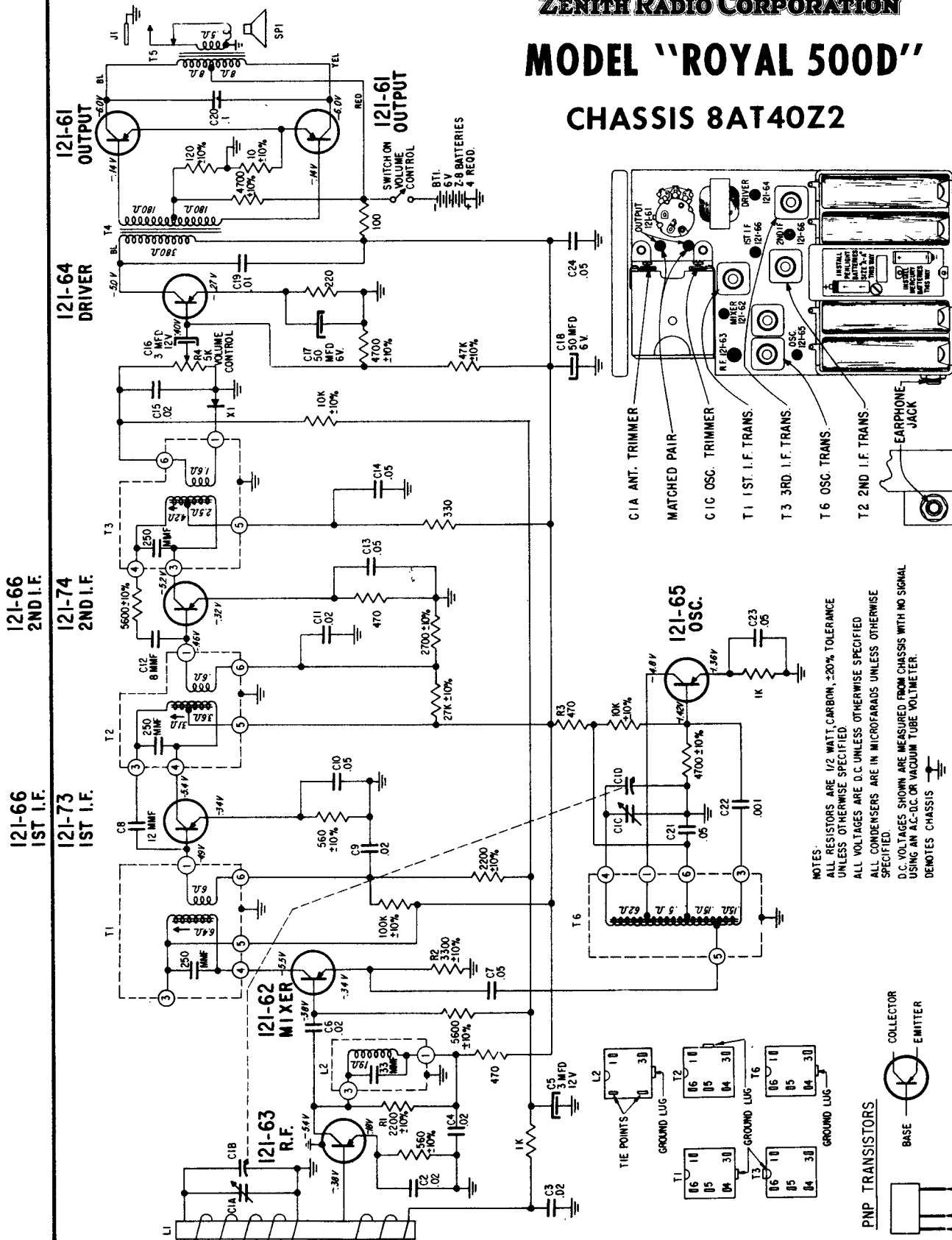
TRANSISTOR & TRIMMER LAYOUT FOR CHASSIS 8AT40Z2 USING 121-66 TRANSISTORS
