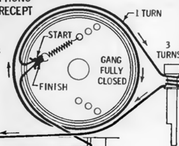
MODEL 5T25-1 ALIGNMENT ADJUSTMENTS AND PARTS LOCATIONS
