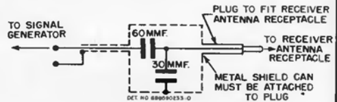
DUMMY ANTENNA DETAIL
