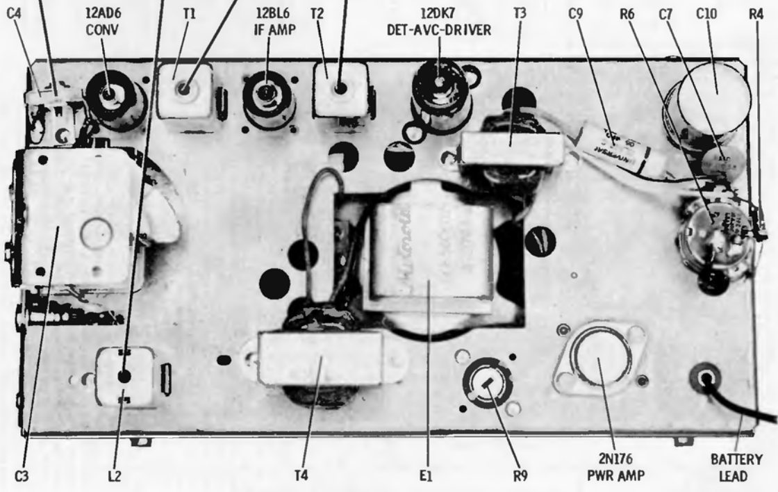
ALIGNMENT ADJUSTMENTS AND PARTS LOCATIONS
