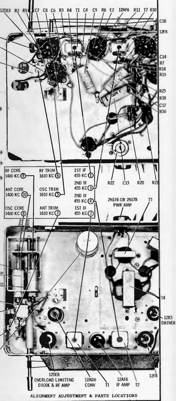
ALIGNMENT ADJUSTMENT & PARTS LOCATIONS
