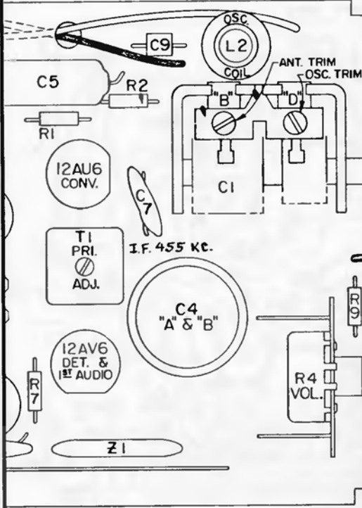
TOP VIEW OF CHASSIS
