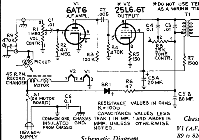
Schematic Diagram Chassis No. RS-152A
