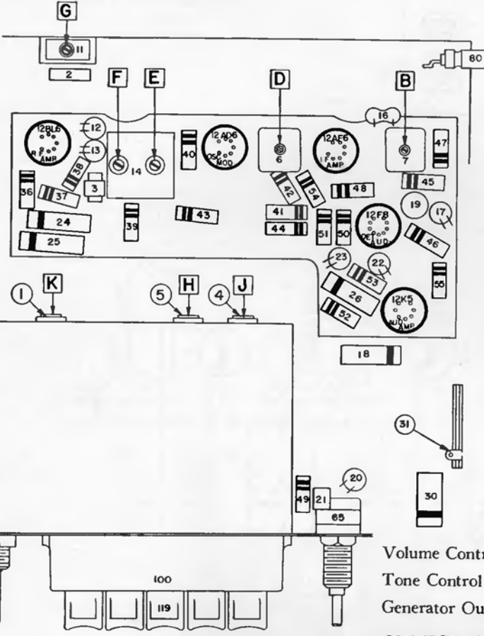
PARTS LAYOUT—TUBE VIEW
