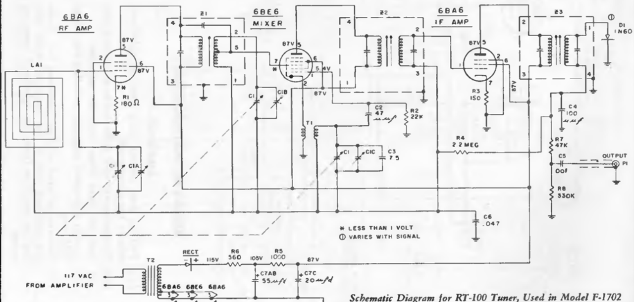
Schematic Diagram for RT-100 Tuner, Used in Model F-1702
