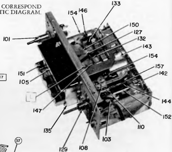
TUNER
