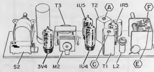
Figure 3. Top View of Chassis 4W2. Tube Locations and Alignment Points Shown.
