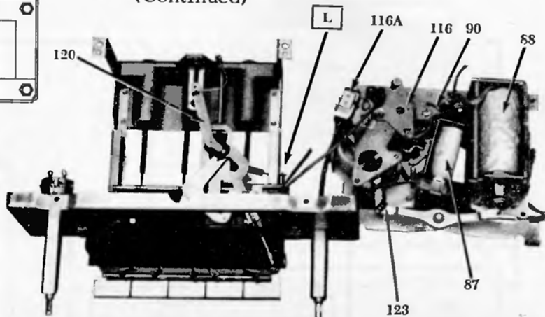
TUNER UNFOLDED
