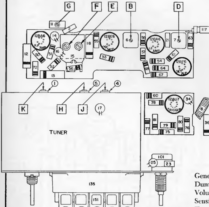
PARTS LAYOUT—TUBE VIEW
