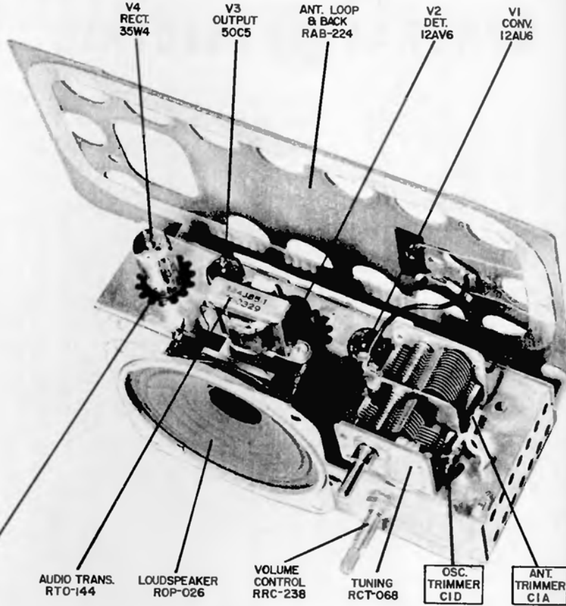
Identification of Components, Top View
