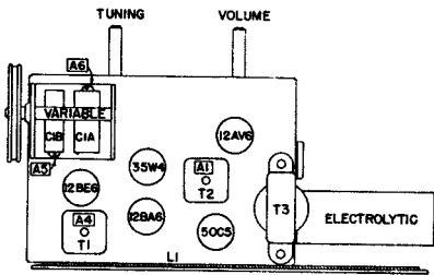
TUBE LAYOUT
