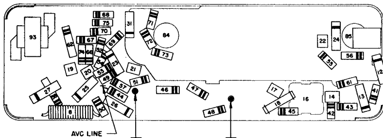
PARTS LAYOUT—CHASSIS VIEW
