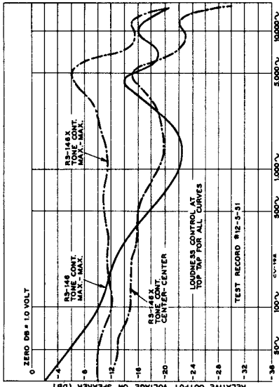
Overall Frequency Response using Test Record
