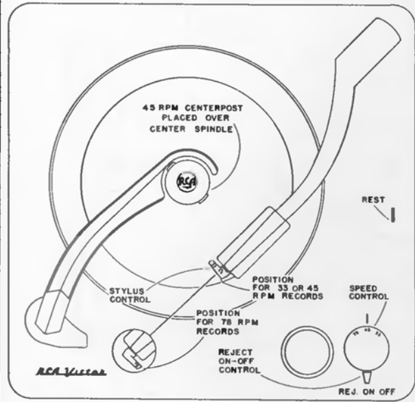
Figure 1—Controls
