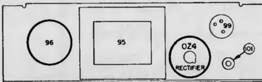
PARTS LAYOUT — TUBE VIEW (POWER SUPPLY)
