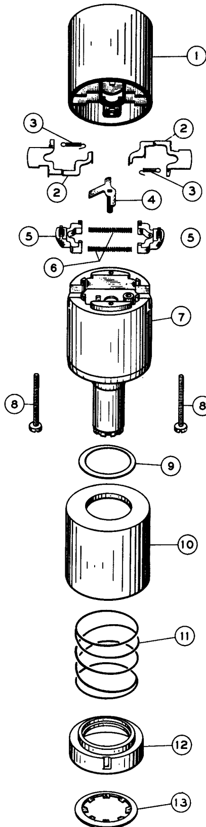
Figure 8—45 r.p.m. Centerpost
