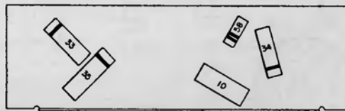
PARTS LAYOUT — CHASSIS VIEW (POWER SUPPLY)
