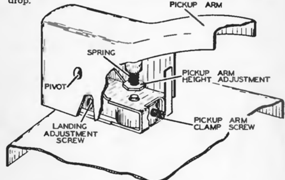
Fig. 3—Pickup Arm Height and Landing Adjustments
