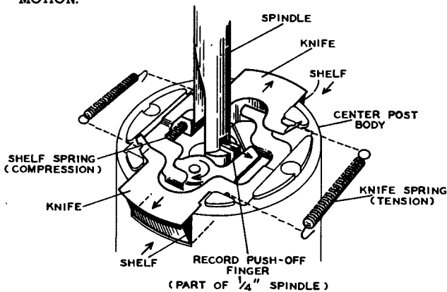
Figure 7—Centerpost Operation
