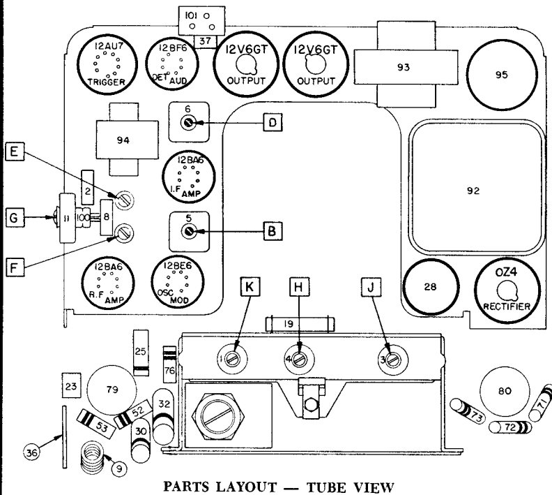
PARTS LAYOUT — TUBE VIEW
