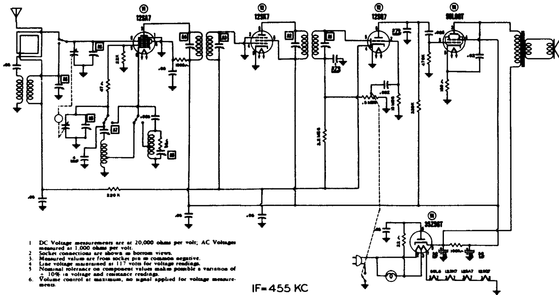
VOLTAGE MEASUREMENTS
