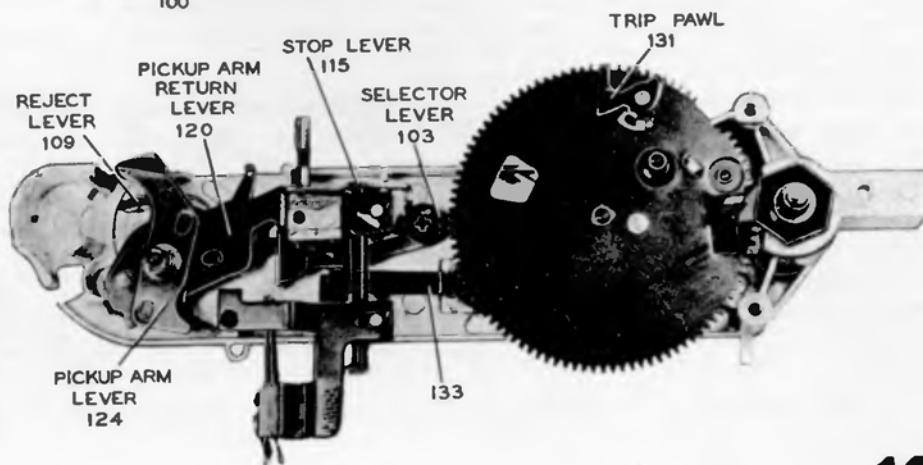
Figure 4— Slide Assembly (View with Slide Removed)
