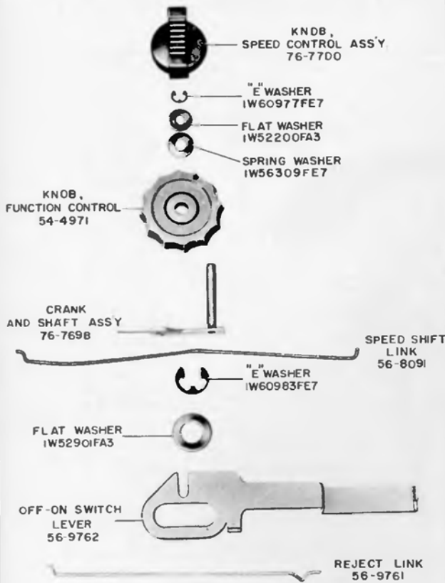
Figure 10. Control Assembly
