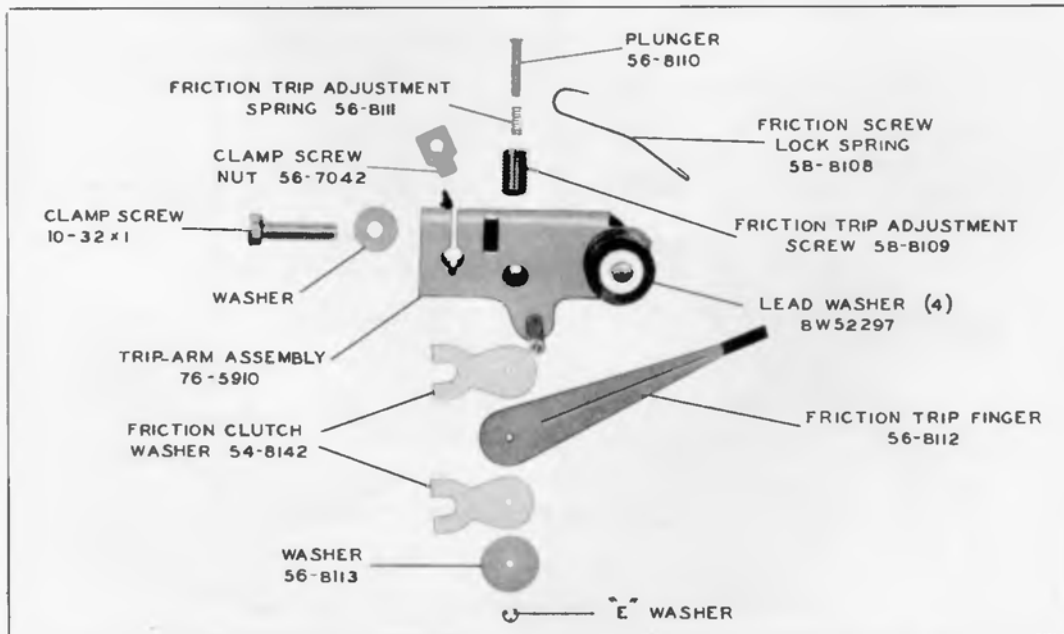
Figure 15. Trip-Arm Assembly
