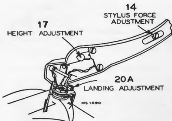
Figure 2—Adjustments
