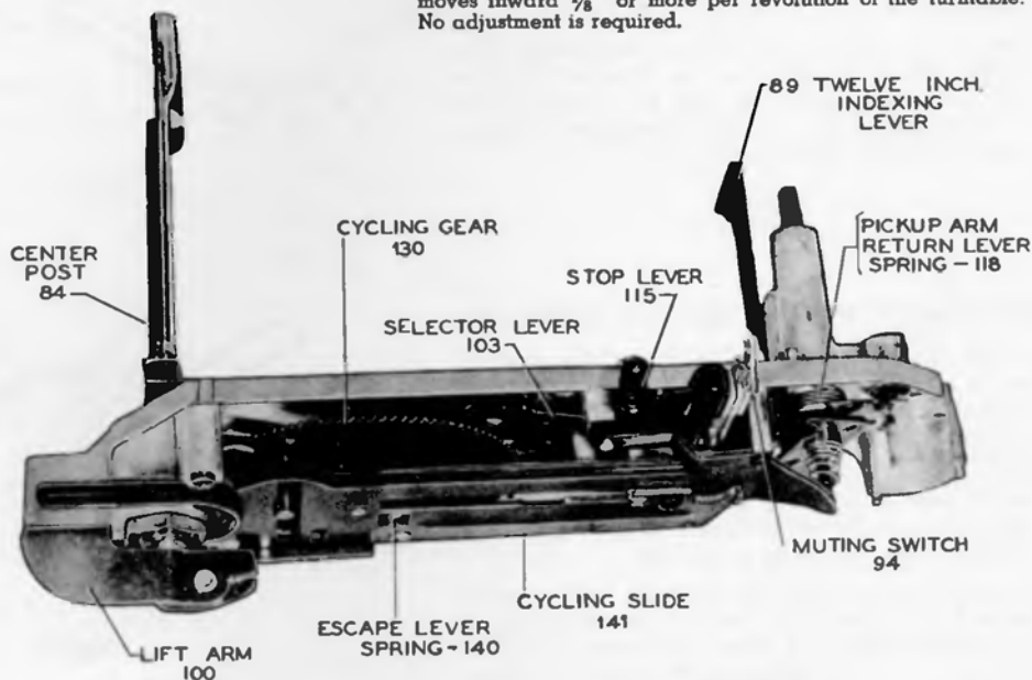
Figure 2—Adjustments
