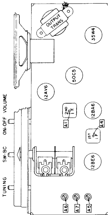
TUBE LAYOUT
