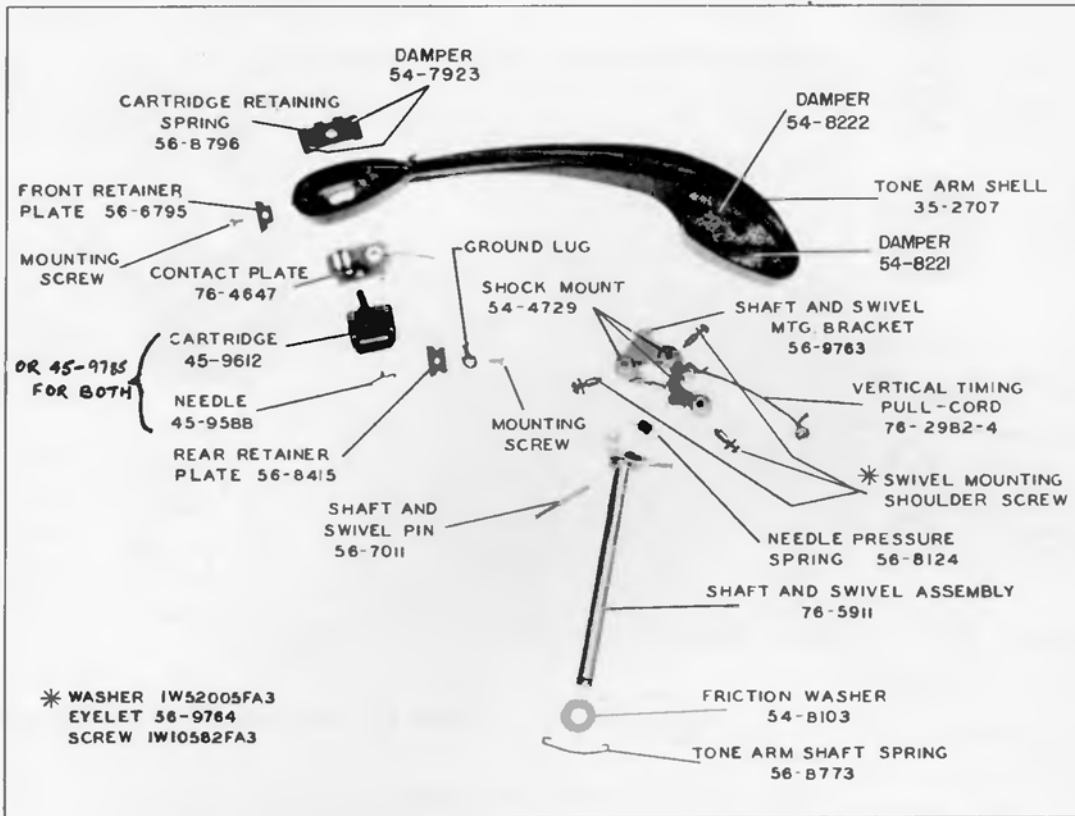
Figure 14. Tone-Arm Assembly
