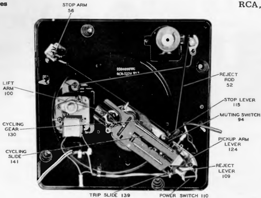
Figure 1—Bottom View
