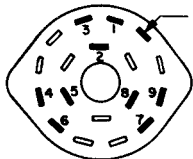
POSITION OF TERMINALS SWITCH S-1
