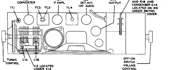
Figure 2. Top View, Showing Tuning Adjustments
