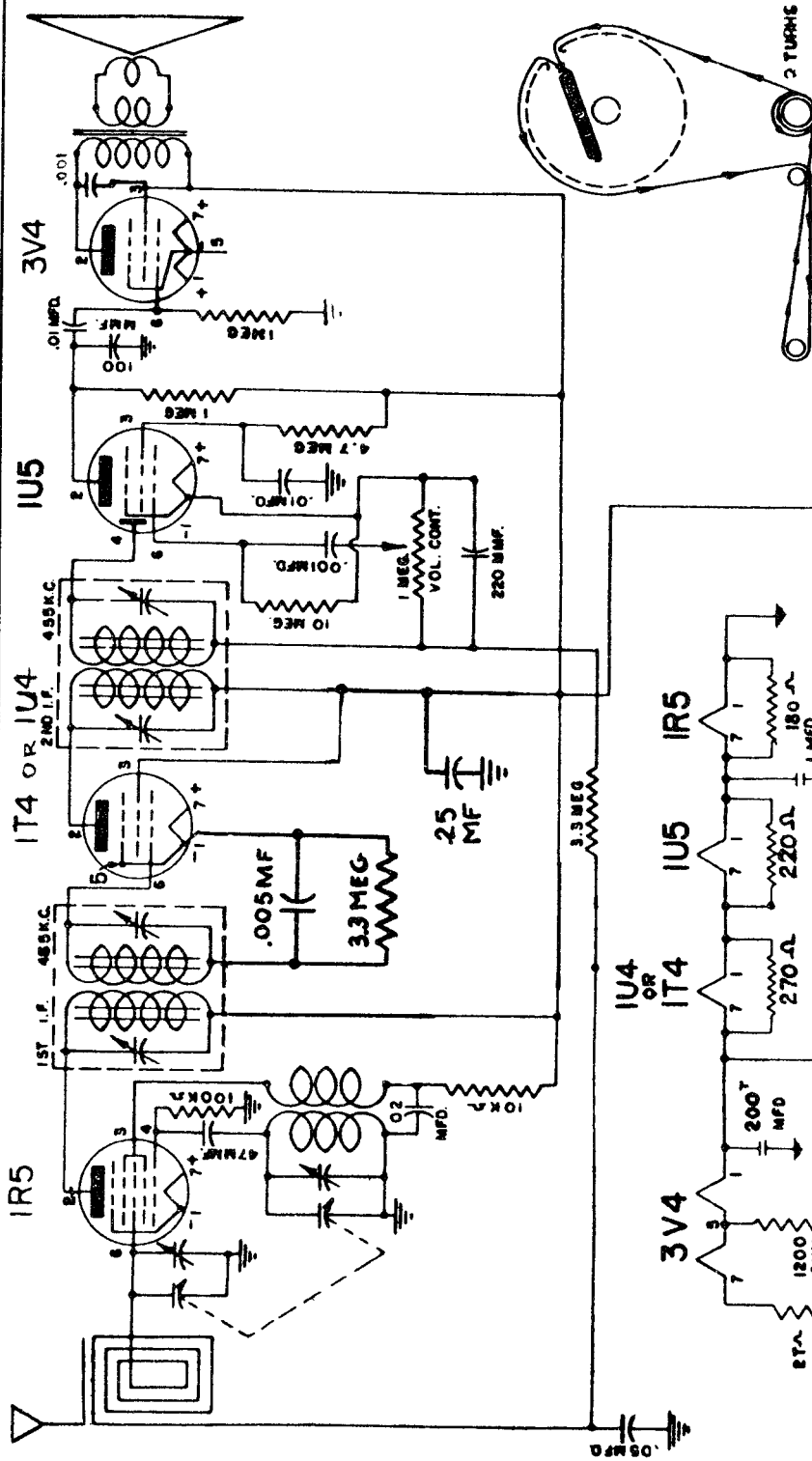
STRINGING DIAGRAM
