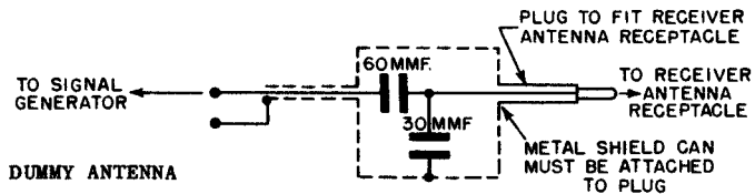
DUMMY ANTENNA
