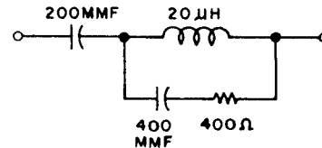
Fig. 7. RTMA Dummy Antenna
