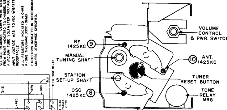
MODEL BT-2 TUBE & TRIMMER LOCATIONS
