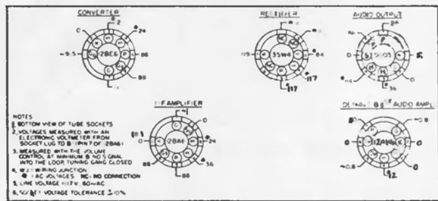
ALIGNMENT CHART
