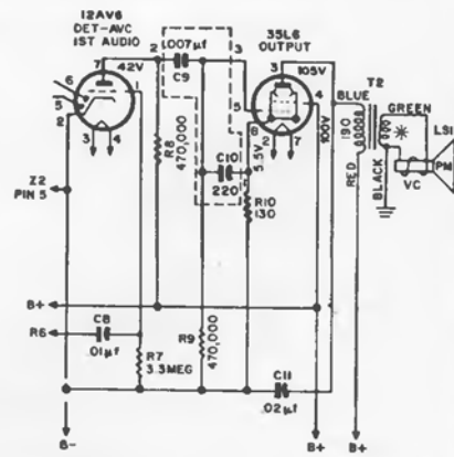
Models 52-543, 52-545,-and 52-547, Output Circuit
