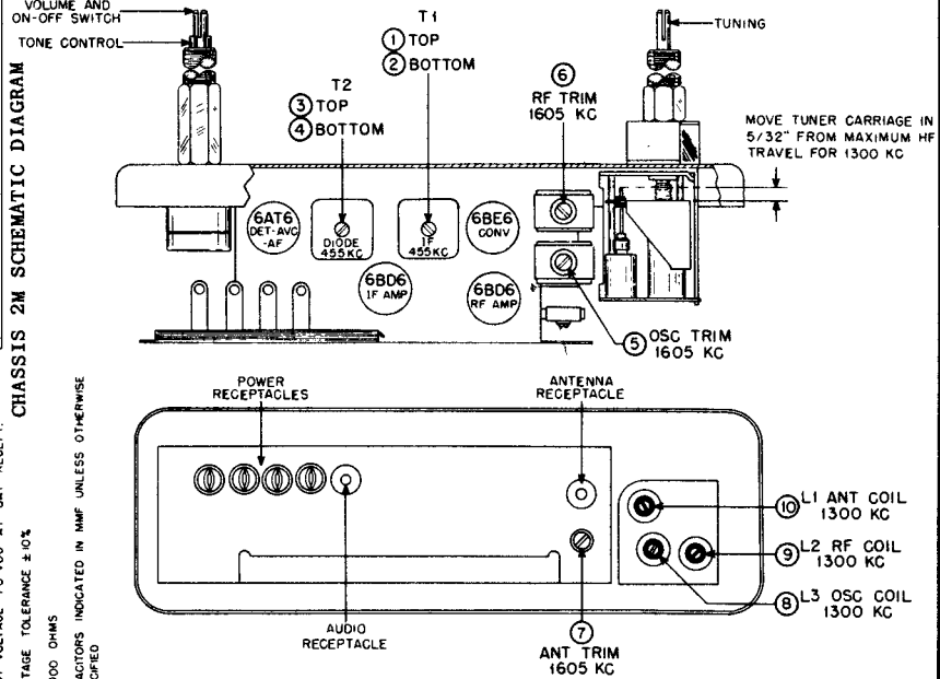
CHASSIS 2M TUBE AND TRIMMER LOCATIONS
