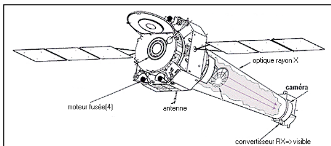
Satellite CHANDRA.
