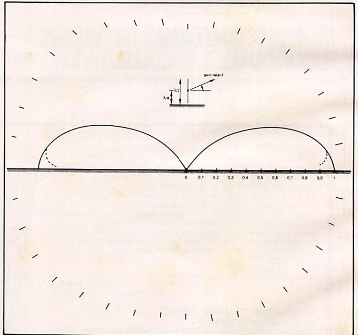
Figure IV.3.1c. - h = \lambda/4 .
