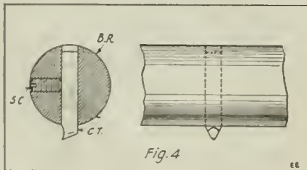
Fig. 4 How the Boring Tool is Made: a Self-Hardening Tool Steel Point is Fitted Slidably in a Hole in the Boring Bar. The Point May Be of Square or Round Stock.
