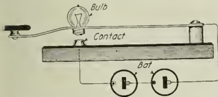
Improved Code Practise Instrument.
