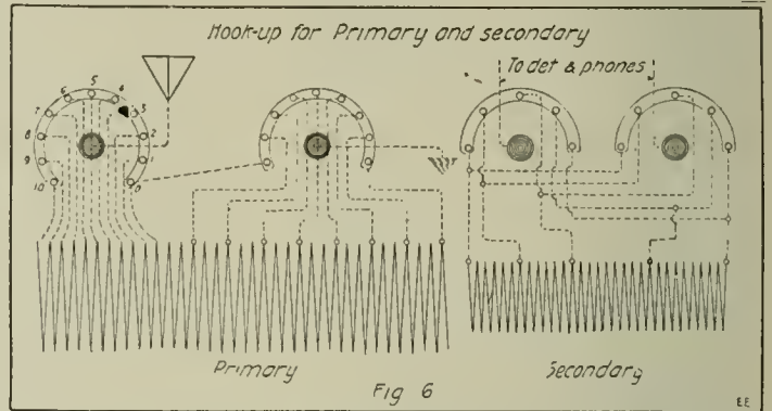
Hook-Up of Primary and Secondary Windings On Vertical Coupler. Note That Secondary Switching Circuit Permits of Reversing the Polarity of the Circuit.
