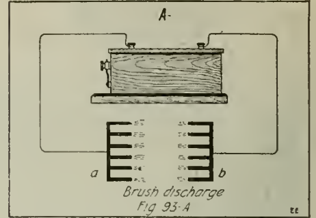
A Brush Discharge is Composed of Many Fine Sparks, Forming an Effluve.
