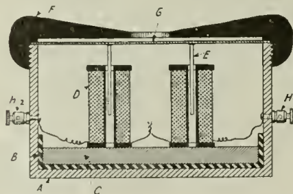
Novel Idea in Telephone Receiver Design.
