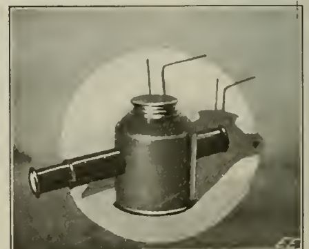
Finished Super-Sensitive Electroscop for the Measurement of Radio-Activity. It is Made from an Oil Can.
