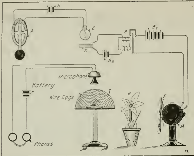
No Buzzer Gives a True Musical Note—But the Bumble-bee Does! Hence, Combine the Bee, a Fan to Waft, Periodically, an Aroma of Hyacinth His Way, When We Have a Pure Musical Note Producer. The Microphone Carries His Tuneful Buzzings to Our Ears, Via the Telephone Receivers.
