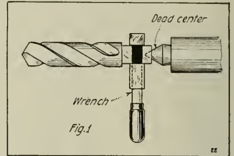
Fig. 1 Holding a Twist Drill in the Lathe by Means of a Monkey Wrench. The Back of the Drill is Placed on the Tail-stock Center.
