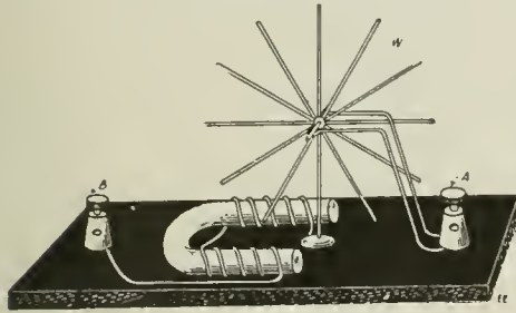
Barlow's wheel Fig. 6
