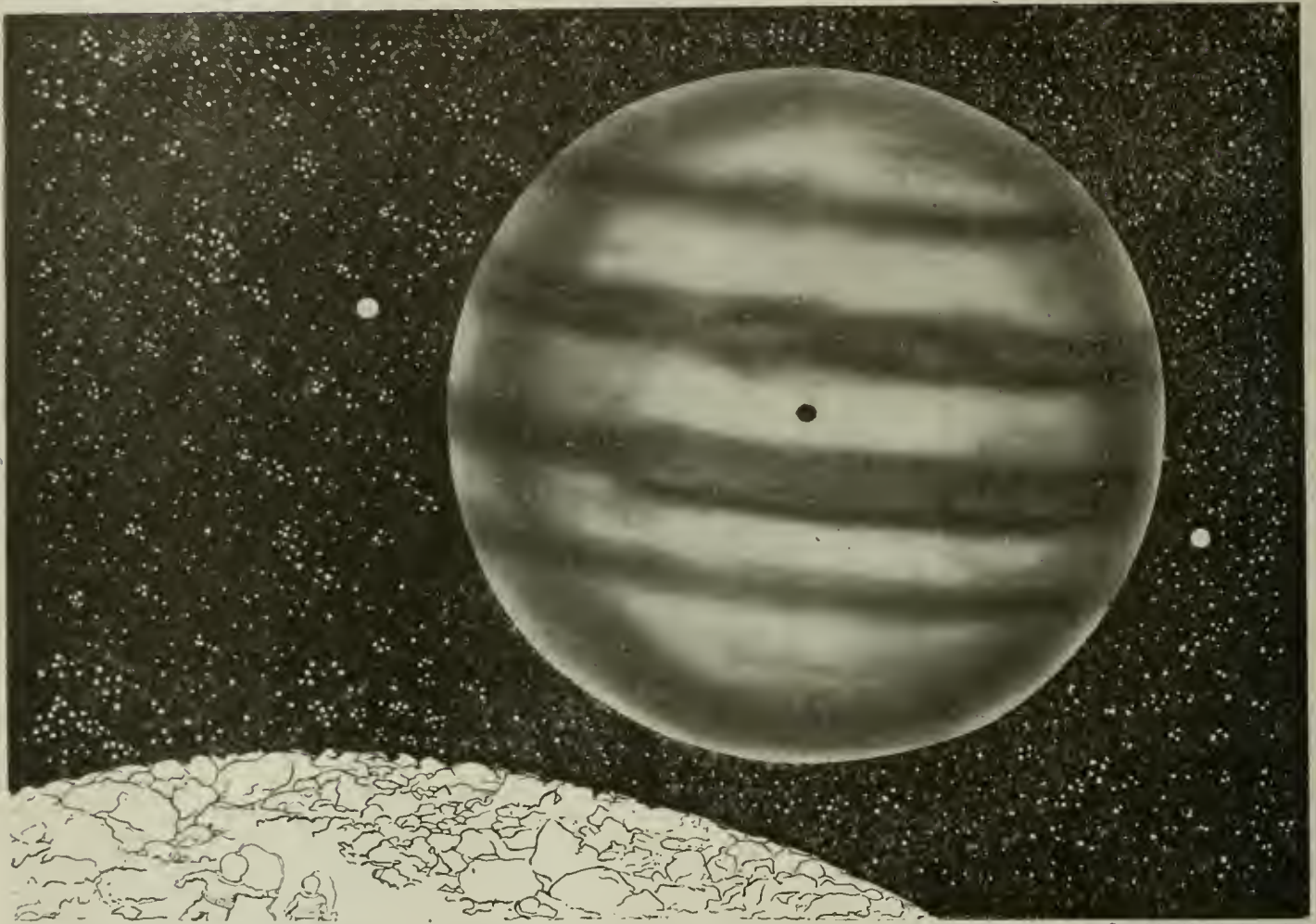
Copyright, 1918, by E. P. Co. Jupiter as Seen from Its Nearest Moon—Satellite V. This Tiny Moon Is Only 67,000 Miles from the Surface of Jupiter. Its Diameter Is Less Than 100 Miles. The Black Spot on the Face of Jupiter Is the Shadow of Another Moon Projected onto the Giant Planet.
