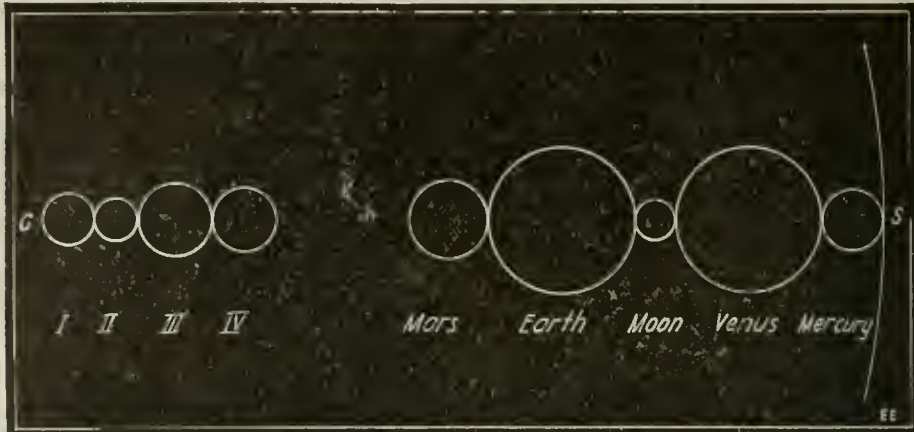
Diagram 1.—Showing the Relative Sizes of the Four Moons of Jupiter, Io, Europa, Ganymede and Callisto, or Satellites I, II, III and IV Respectively, and the Moon and Terrestrial Planets Mercury, Venus, Earth and Mars. The Distance from C to S is the Distance from the "Center" to the "Surface" of Jupiter. So if All the Satellites of the Planet and the Terrestrial Planets and Moon Were Placed Side by Side Their Combined Diameters Would Fall Short of the Surface of the Planet by a Distance About Equal to the Diameter of the Earth.
