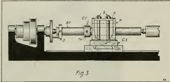
Fig. 3 Boring Out a Casting in the Lathe by Means of a Boring Bar "BR." The Casting is Secured by Bolts "B" to the Saddle "CS."
