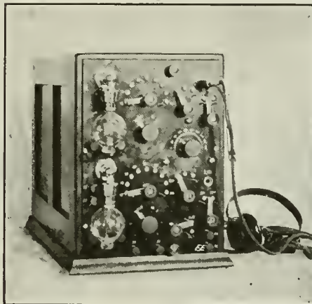
Fig. 2. New Combination Audion, Ultra-audion and One-Step Amplifier Designed By de Forest.
