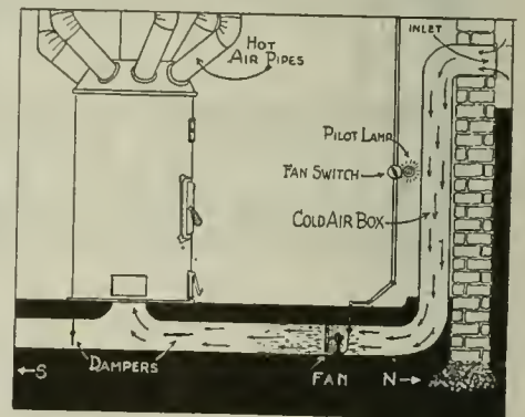
To Improve the Cold Air Box Draft To Your Furnace, Install An Electric Fan in the Draft Passage After the Manner Illustrated. A "North" and "South" Cold Air Box, Fitted With Suitable Cut-Off Dampers, Makes a Very Dependable Furnace, No Matter Which Way the Wind Blows.
