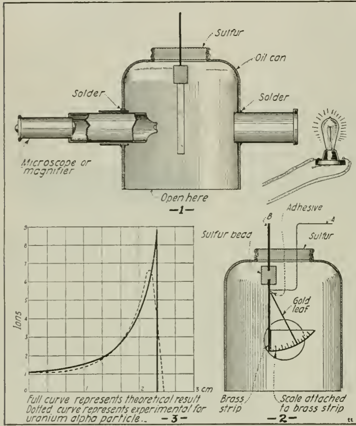
The Most Important Property Possessed by the Radiations of Radio-Active Substances Is the Power of Discharging Electrified Bodies. Hence, the Discharge of an Electroscop Placed in the Vicinity of the Radio-Active Substance, Furnishes an Efficient Means of Measuring the Intensity of the Activity.
