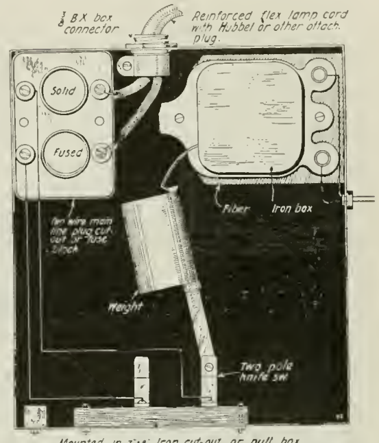
Construction of "Remote Control" Switch Which Can Be Made With a Buzzer or Bell Movement to Trip the Weighted Knife Switch Blade.
