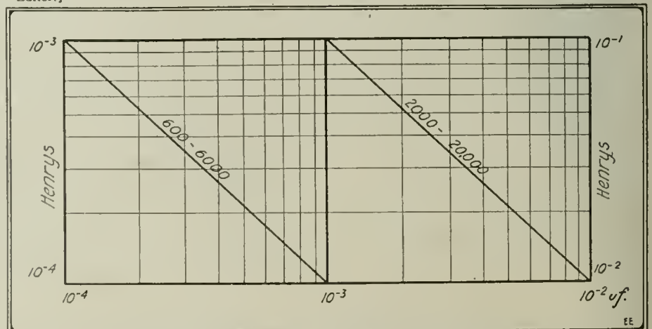
For All Ordinary Radio Calculations This Simplified Graph Fills the Bill as Well as the Larger One Published in the September Issue. It Gives the Value of Inductance and Capacity for Wave Lengths from 600 to 20,000 Meters.
