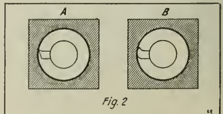
Fig. 2 Proper Clearance on Boring Tool (Left) and Improperly Ground Tool at Right.
