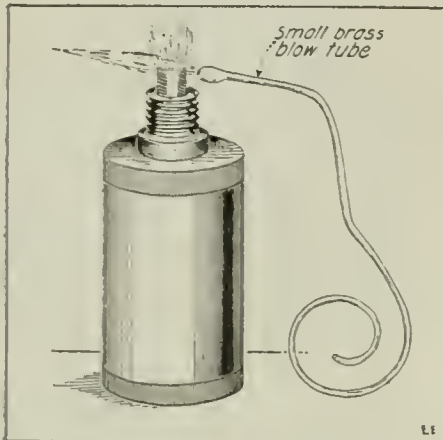
Simply Fill a Fan Grease Cup with Wood Alcohol, Insert a Wick in the Hole, and You Have a Serviceable Little Spirit Lamp for Light Soldering
