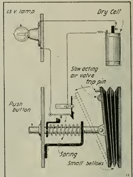
Here is the Secret of the Automatic Cut-off Mechanism of the Flashlight that Opens Its Lamp Circuit After Burning for a Minute. A Small Air Bellows Does the Trick.
