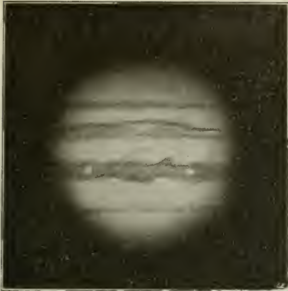
Jupiter Photographed October 19, 1915, with the 24-Inch Refractor by E. C. Slipher of the Lowell Observatory.
