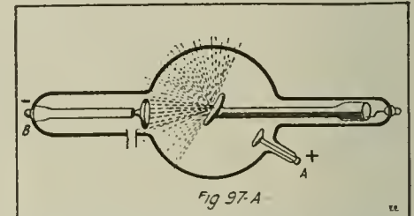
Fig. 97-A. For the Production of Concentrated X-Rays, a Special Form of Focus Tube is Used. Cathode Rays Coming from the Concave Electrode at Left, Converge and Strike Platinum Target at Right, Where X-Rays Are Generated.
