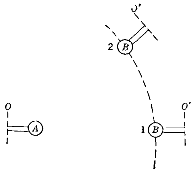
FIG. 2-13.—On the pattern reciprocity theorem.
