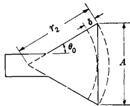
FIG. 10-14.—Origin of phase variation across the aperture of a sectoral horn ( \Delta\phi = 2\pi\delta/\lambda_0 ).
