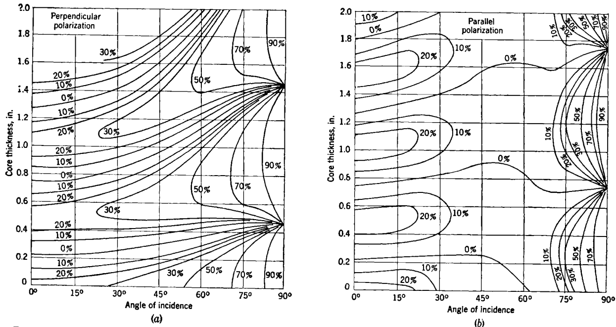
FIG. 14.17.—Typical charts showing contours of constant reflection as a function of core thickness and angle of incidence for the following conditions: \lambda_0 = 3.2 cm; core \epsilon'/\epsilon_0 = 1.4 ; skin \epsilon'/\epsilon_0 = 3.7 ; skin thickness = 0.050 in. (a) Polarization perpendicular to the plane of incidence; (b) parallel polarization.
