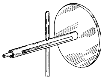
FIG. 8-12.—Dipole-disk feed.
