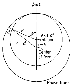
FIG. 15-10.—Center of feed correction. Pickup moves on circle of radius R . True wavefront is circle of radius r . Reference point \psi = 0 .
