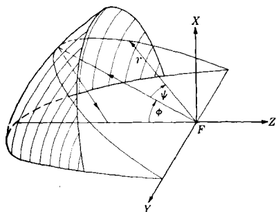
FIG. 13-33.—Double curvature surface and spherical coordinate system.
