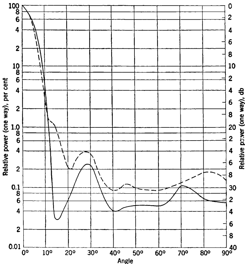
FIG. 12-10.—Principal plane patterns of 30-in.-diameter paraboloid ( f/D = 0.354 ; illuminated by the dipole-disk feed; \lambda = 10 cm; — E -plane; - - - H -plane; \Theta_E = 10.2^\circ ; \Theta_H = 9.5^\circ .)
