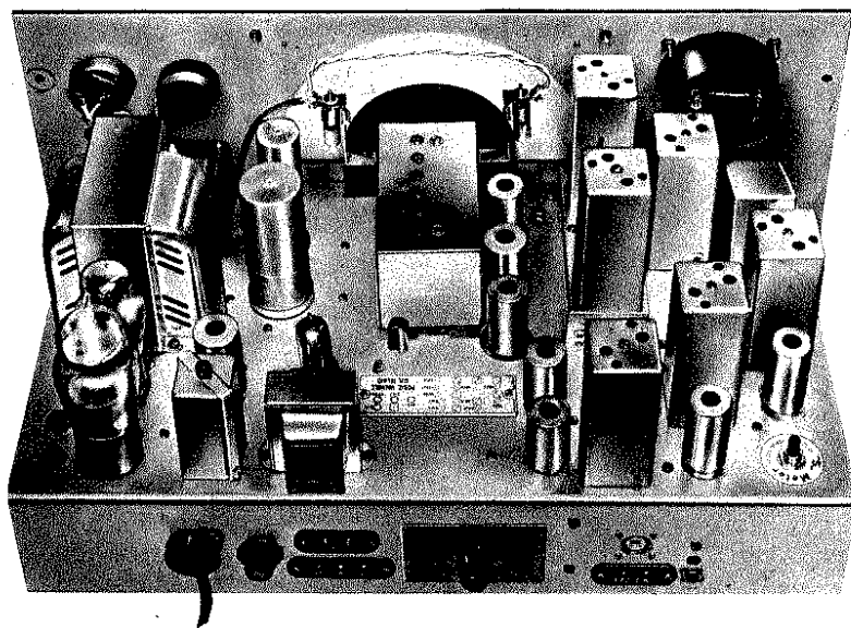
View of the chassis of the G 207. On the rear side of the chassis one can observe, from left to right: the line voltage selector switch; the fuse; the terminal strip (2-pin) for remote control; the terminal strip (3-pin) for loud speaker connection; the shielded antenna terminal; and, finally, the ground terminal.
